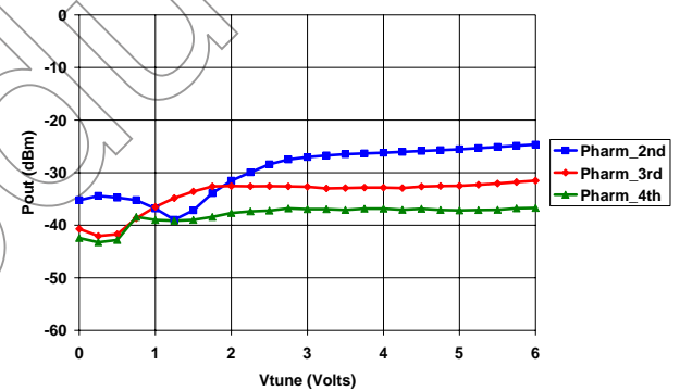
XQ1004-BD Harmonic Levels vs. Tuning Voltage
